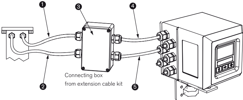
Sensor fitting Type S051 with junction box
